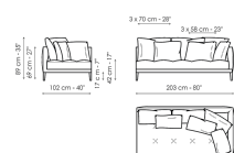
End section corner sofa 203
